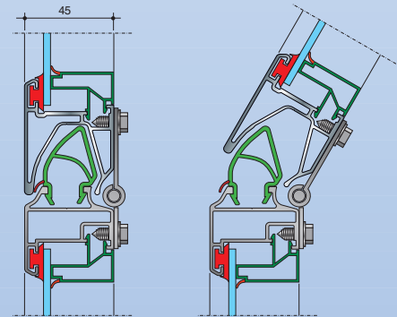
Finger pinch protection detail
